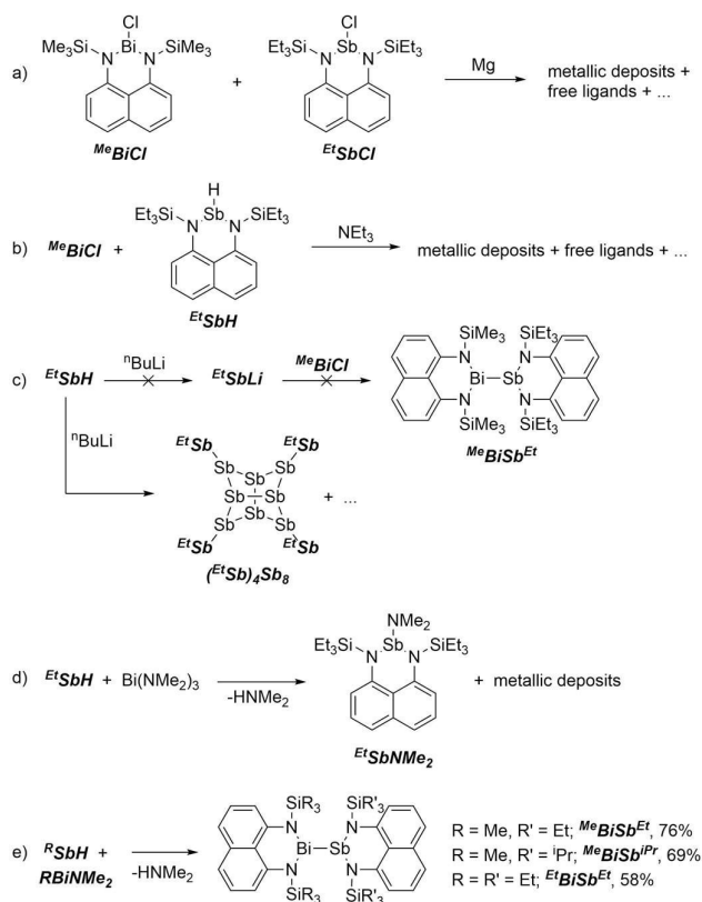
Scheme 2 Synthesis of (EtSb)_4Sb_8 and derivatives of R'Sb^R .
