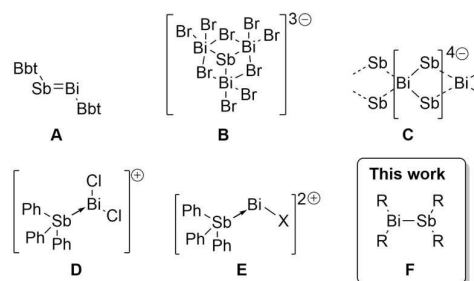
Scheme 1 Isolated compounds containing Bi–Sb bonds. See text for references. Bbt = o,o -( \text{CH}(\text{SiMe}_3)_2 ) 2 - p -C( \text{SiMe}_3 )-Ph.
