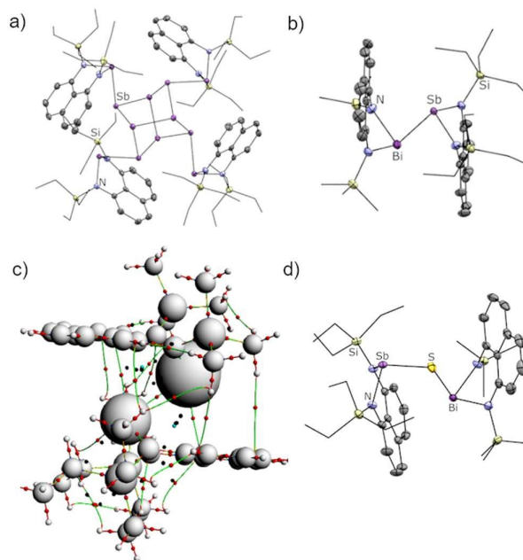
Fig. 1 a) Single-crystal X-ray structures of (EtSb)_4Sb_8 . b) Single-crystal X-ray structures of MeBiSb^{Et} . Selected bond lengths (Å) and angles (°): Bi-Sb 2.9775(9), Bi-N 2.161(4) and 2.161(4), Sb-N 2.059(4) and 2.059(4), N-Bi-N 83.6(2), N-Sb-N 87.6(2) c) AIM calculated bond paths and critical points for MeBiSb^{Et} . White spheres denote the nuclear basins (atoms). The vertical green lines evidence bonding interactions between the ligands in the periphery of the Bi-Sb bond. d) Single-crystal X-ray structures of MeBiSb^{Et} . Selected bond lengths (Å) and angles (°): Sb-S 2.3838(8), Bi-S 2.5456(7), Bi-N 2.141(2) and 2.150(2), Sb-N 2.040(2) and 2.045(2), N-Bi-N 83.86(8), N-Sb-N 89.35(8). Thermal ellipsoids are shown at the 50% probability level. Hydrogens have been omitted and silyl groups are shown in wireframe for clarity.
