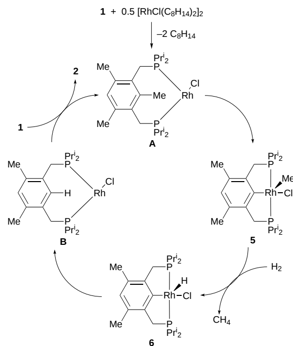
Scheme 3 Proposed catalytic hydrogenolysis cycle for 1 with rhodium
