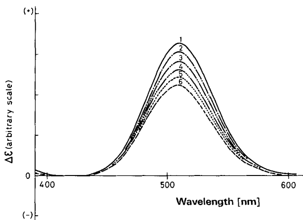
Fig. 2. CD-spectral change with photo-irradiation time of optically active isomer ( \Delta-(+)_589-[Co(gly)(en)_2]^{2+} ) in the presence of racemic [Ru(bpy)_3]^{2+} . [[Co(gly)(en)_2]^{2+}] = 1.00 \times 10^{-2}M ; [[Ru(bpy)_3]^{2+}] = 1.00 \times 10^{-5}M ; [en] = 2.00M ; [OH^-] = 1.58 \times 10^{-2}M (buffered); [Cl^-] = 1.0M ; 25^\circ . Irradiation wavelength, 452 nm. Irradiation time, 1: 0; 2: 60; 3: 120; 4: 180; 5: 240; and 6: 300 min. No change in CD spectra was noticed in the absence of [Ru(bpy)_3]^{2+} .
