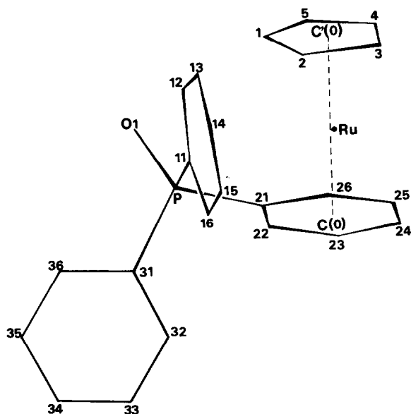
Fig. 2. Molecular structure and atom numbering of [\text{Ru}((\eta^6\text{-C}_6\text{H}_5)\text{Ph}_2\text{PO})(\eta^5\text{-C}_5\text{H}_5)]\text{ClO}_4 .
