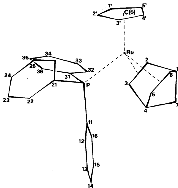
Fig. 1. Molecular structure and atom numbering of [\text{Ru}(\text{nbd})(\text{PPh}_3)(\eta\text{-C}_5\text{H}_5)]\text{ClO}_4 .
