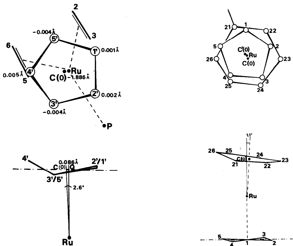
Fig. 3. The coordination of the Ru atoms in compounds VIII and X as projected normal to the cyclopentadienyl rings.
