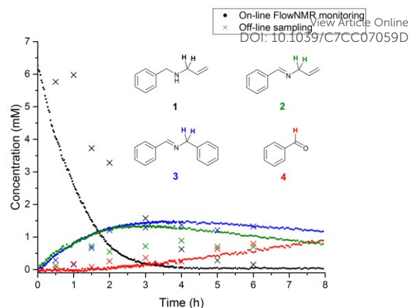
Figure 2: Off-line and on-line FlowNMR reaction profiles of N-allylbenzylamine ( 1 ) in MeCN (6.4 mM) at 20°C in the presence of Eosin Y catalyst (1 mol%) under green LED illumination (633 \mu W) to form 2 , 3 and 4 . (On-line: 100 mL, 4 mL min -1 flowrate, WET solvent suppression, 1.64 s acquisition time, 3 s relaxation delay, 12 scans. Off-line: 300 mL, 3 s acquisition time, 1 s relaxation delay, 16 scans. 20 mL samples were periodically withdrawn from the reaction mixture and concentrated under reduced pressure before dissolving in CDCl 3 for analysis). See the supporting information for details.
