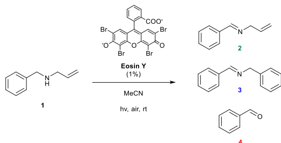
Scheme 1: Structure of Eosin Y and photocatalytic oxidation of allylic amines.
