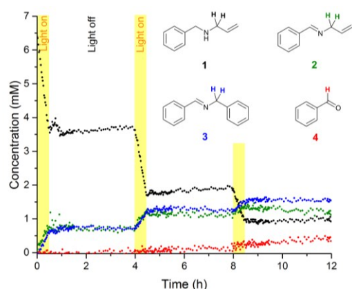
Figure 4: ^1\text{H} FlowNMR reaction profiles of N-allylbenzylamine ( 1 ) in MeCN (6.4 mM) at 20^\circ\text{C} in the presence of Eosin Y catalyst (1 mol%) under chopped green LED illumination ( 633\text{ }\mu\text{W} ) to form 2 , 3 and 4 (100 mL, 4\text{ mLmin}^{-1} flowrate, WET solvent suppression, 1.46 s acquisition time, 3 s relaxation delay, 12 scans).
