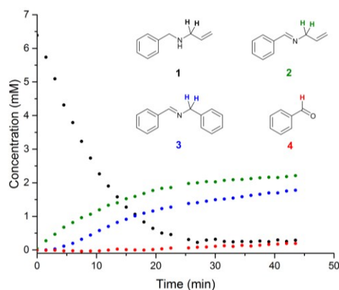
Figure 1: ^1\text{H} FlowNMR reaction profiles of N-allylbenzylamine ( 1 ) in MeCN (6.4 mM) at 0^\circ\text{C} in the presence of Eosin Y catalyst (1 mol%) under halogen light illumination (250 mW) to form 2 , 3 and 4 (200 mL, 4\text{ mLmin}^{-1} flowrate, WET solvent suppression, 4 s acquisition time, 1 s relaxation delay, 16 scans).
