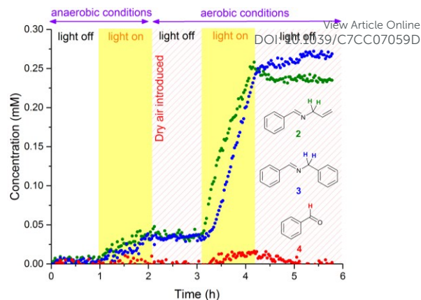
Figure 5: ^1\text{H} FlowNMR reaction profiles of N-allylbenzylamine ( 1 ) in MeCN (6.4 mM) at 20^\circ\text{C} in the presence of Eosin Y catalyst (1 mol%) under chopped green LED illumination ( 633\text{ }\mu\text{W} ) and different atmospheres (argon to dry air) to form 2 , 3 and 4 (50 mL, 4\text{ mLmin}^{-1} flowrate, WET solvent suppression, 1.46 s acquisition time, 3 s relaxation delay, 16 scans).
