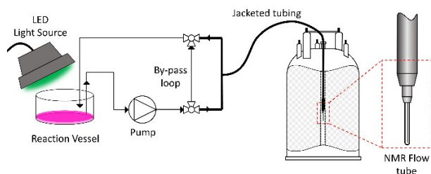
Figure 1: FlowNMR setup for monitoring photochemical reactions (not to scale).
