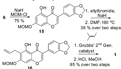
SCHEME 4. Completed Synthesis of Derrubone
