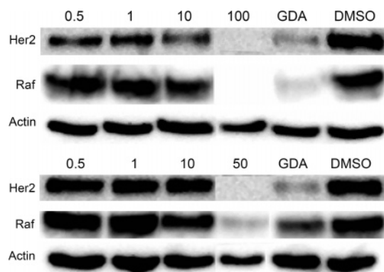
FIGURE 3. Western blot analysis of 14 (top) and 22c (bottom) in MCF-7 cells ( \mu M). Geldanamycin (500 nM) was used as the positive control.
