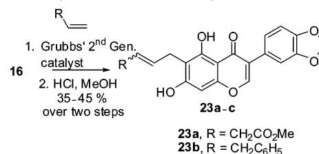
SCHEME 6. Synthesis of C6 Analogues
