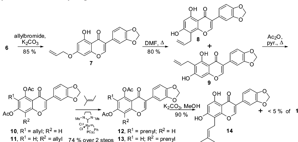
SCHEME 4. Completed Synthesis of Derrubone
