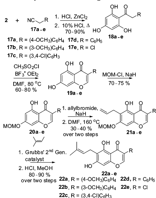
SCHEME 6. Synthesis of C6 Analogues
