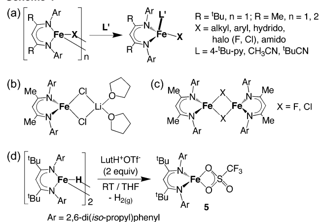
Figure 2. Examples of four-coordinate iron(II) diketiminate complexes with trigonal planar distortions. Molecular structures of the new complexes \text{L}^{\text{Me}}\text{Fe}^{\text{II}}\text{Bu}^{\text{I}}(\text{BuCN}) (1) (a) and \text{L}^{\text{Me}}\text{Fe}^{\text{II}}\text{CH}_2\text{Bu}^{\text{I}}(\text{BuCN}) (2) (b). Thermal ellipsoids are shown at 50% probability with hydrogen atoms omitted for clarity. The pseudooxalal (axial) position in each complex is occupied by the neutral ligand trimethylacetanitrile ( \text{L}^{\text{I}} ).
