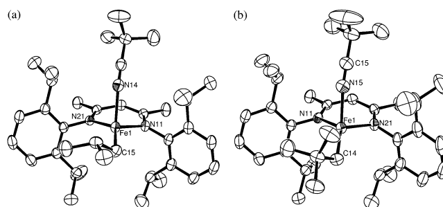
Figure 2. Examples of four-coordinate iron(II) diketiminate complexes with trigonal planar distortions. Molecular structures of the new complexes \text{L}^{\text{Me}}\text{Fe}^{\text{II}}\text{Bu}^{\text{I}}(\text{BuCN}) (1) (a) and \text{L}^{\text{Me}}\text{Fe}^{\text{II}}\text{CH}_2\text{Bu}^{\text{I}}(\text{BuCN}) (2) (b). Thermal ellipsoids are shown at 50% probability with hydrogen atoms omitted for clarity. The pseudooxalal (axial) position in each complex is occupied by the neutral ligand trimethylacetanitrile ( \text{L}^{\text{I}} ).
