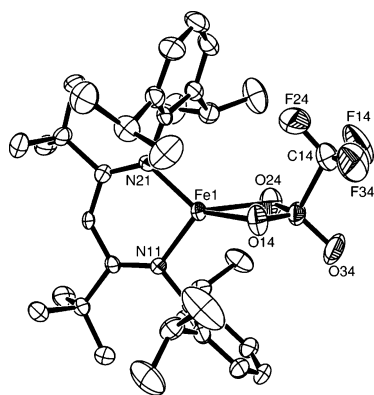
Figure 4. Thermal ellipsoid plot of the X-ray crystal structure of L tBu -Fe(η 2 -OTf) ( 5 ). Thermal ellipsoids are shown at 50% probability. Hydrogen atoms are omitted for clarity.
