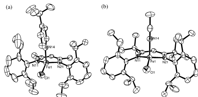
Figure 3. Molecular structures of the new four-coordinate diketimate iron(II) chloride complexes L^{\text{Me}}\text{FeCl}(4\text{-Bu-py}) ( 3 ) and L^{\text{Bu}}\text{FeCl}(\text{CH}_3\text{CN}) ( 4 ). Thermal ellipsoids are drawn at 50% probability with hydrogen atoms omitted for clarity. The pseudoapical (axial) positions are occupied by 4- tert -butylpyridine and acetonitrile, respectively.
