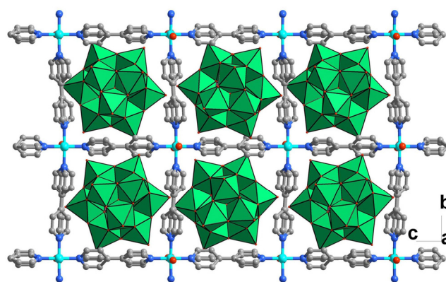
Fig. 5 Crystal structure of CR-BPY2 showing the stacking pattern of the grid-like sheets with [\text{SiW}_{11}\text{O}_{39}\text{Ru}(\text{H}_2\text{O})]^{5-} imbedded. The atoms of copper, tungsten, carbon, nitrogen and oxygen were drawn in cyan, green, gray, dark blue and red, respectively.
