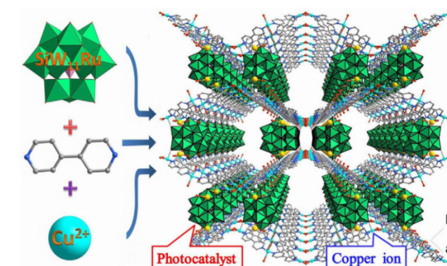
Scheme 1. Synthetic procedure for the 3D CR-BPY1 MOF that is composed of wavy-like Cu-BPY sheets and [SiW 11 O 40 Ru] 7- anions showing the combination of the dual catalytic units and channels for chemical transformations.
