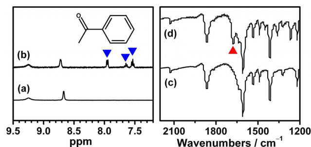
Fig. 4 ^1\text{H} NMR in \text{CDCl}_3/\text{DMSO} and solid state IR spectra of the desolvated CR-BPY1 (a) and (c), respectively, and of the desolvated CR-BPY1 impregnated in a dichloromethane solution of acetophenone (b) and (d), respectively, showing the absorbency and activation of substrate in the MOF. The blue and red triangle represented the signals of acetophenone in the NMR and IR spectra, respectively.
