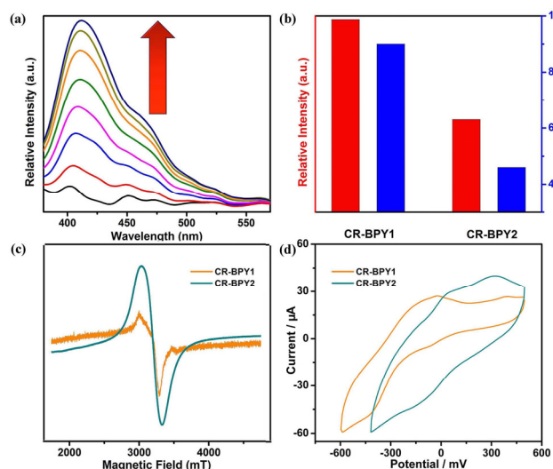
Fig. 3 (a) Family of emission spectra of CR-BPY1 (0.1% in weight) in \text{CH}_2\text{Cl}_2 suspension upon addition of N -phenyl-tetrahydroisoquinoline up to 0.50 mM, excitation at 362 nm. (b) The luminescence intensities of CR-BPY1 and CR-BPY2 upon addition of the same amount of N -phenyl-tetrahydroisoquinoline up to 0.50 mM at room temperature in \text{CH}_2\text{Cl}_2 ; The catalytic activities of CR-BPY1 and CR-BPY2 using N -phenyl-tetrahydroisoquinoline and nitromethane as the coupling partners. (c) EPR spectra of CR-BPY1 ( g = 2.1438 ) and CR-BPY2 ( g = 2.1320 ) in solid state at 77K, respectively. (d) Solid state cyclic voltammetry of CR-BPY1 and CR-BPY2, respectively, scan rate: 50 \text{ mV} \cdot \text{s}^{-1} .
