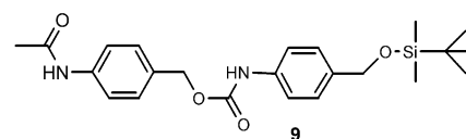
Figure 1. Double spacer-containing model compound 9 .
