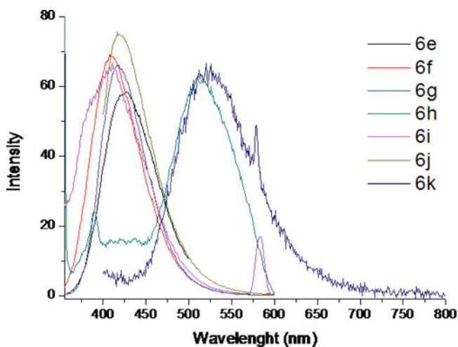
Figure 5. Fluorescence emission spectra of compounds 6e–k in dichloromethane solution. Signal in 582 nm is due to re-absorption of sample.
