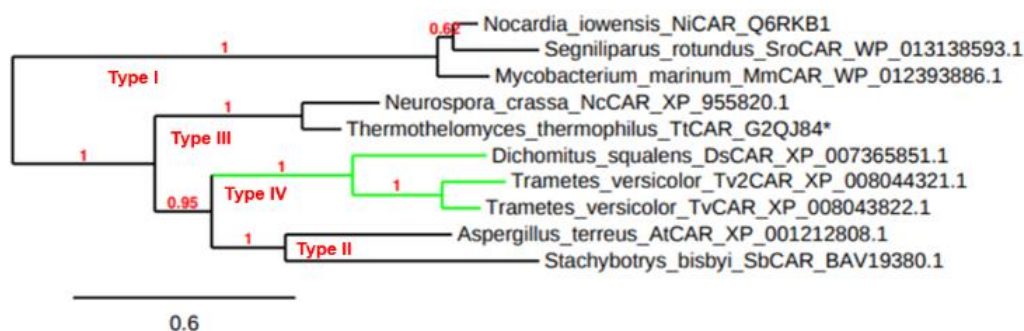
Figure 2. A phylogenetic tree of fungal and bacterial CAR enzymes, categorized in four subtypes. Newly discovered sequences and previously described CARs [8],[14],[15],[18],[19],[23] were incorporated in the phylogenetic analysis. Green branches represent CARs investigated in this study. *TiCAR was identified in Thermotheomyces thermophilus , which is also known as Myceliophthora thermophila , Thielavia heterothallica ATCC 42464, or Sporotrichum thermophile .
