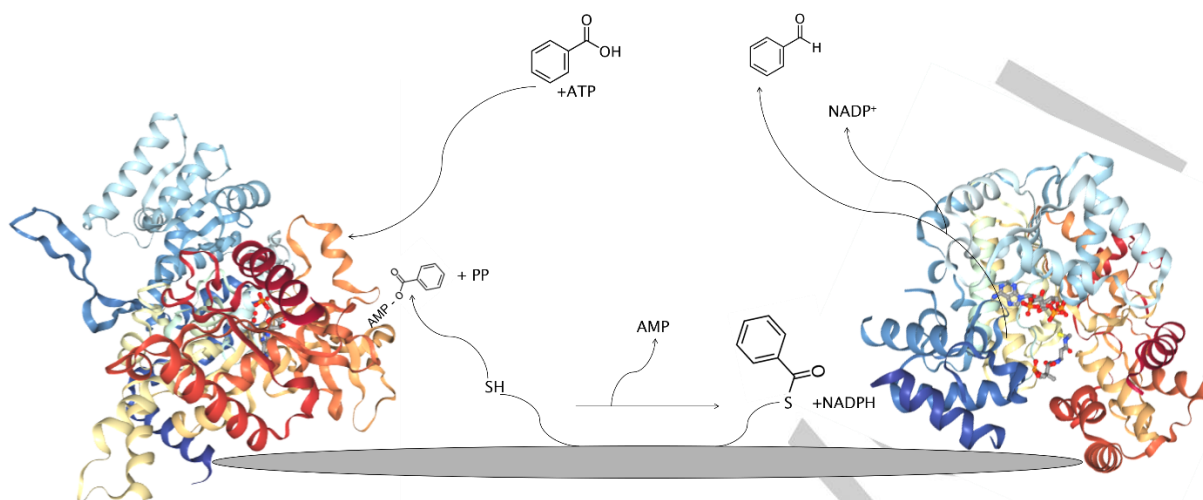
Figure 1. Schematic reaction mechanism of CAR enzymes (E.C.1.2.1.30). Left: ATP and substrate enter the active site of the adenylation domain. The structure of the adenylation domain of Nocardia iowensis CAR (NiCAR) is shown in complex with AMP (PDB ID: 5MSC). [6] The substrate is then activated as an AMP anhydride and pyrophosphate is released. [9] Middle: A thioester is formed at the phosphopantetheine binding site (grey), and AMP is released. Right: the thioester is translocated to the reductase domain (PDB ID: 5MSO). [6] The reductase domain incorporated in the scheme is from Mycobacterium marinum in complex with NADP + . The last step is thioester reduction and release of the aldehyde and NADP + . Microsoft Power Point and ChemDraw were used to generate the figure.
