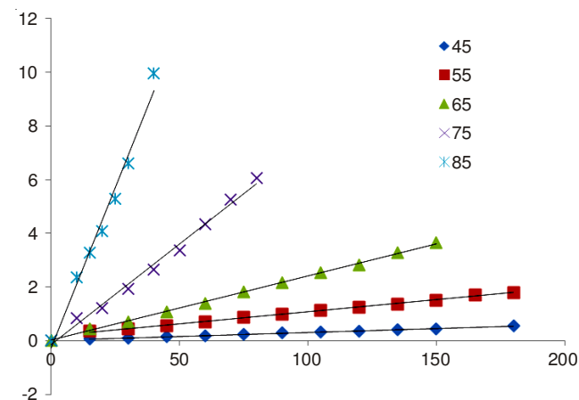
Fig. 2. Kinetic relationship of concentration of chloroacetic acid with time (c-t) at 45-85 °C
