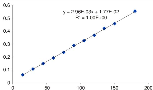
Fig. 1. Kinetic relationship of concentration of chloroacetic acid with time (c-t) at 45 °C
