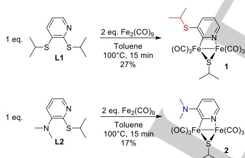
Scheme 1. Synthesis of novel [\text{FeFe}]\text{-H}_2\text{ase} mimics 1 and 2 .
