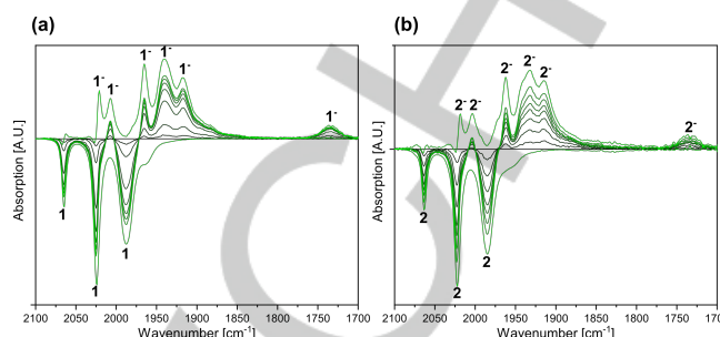
Figure 5. IR spectroscopic changes observed during the reduction of 2 mM 1 (a) and 2 (b) in \text{CH}_3\text{CN} containing 0.2 \text{ M NBu}_4\text{PF}_6 ( 0.001 \text{ V s}^{-1} ).
