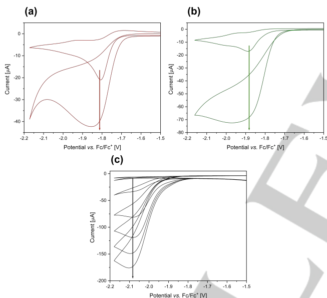
Figure 8. Electrocatalytic reduction of PhOH. (a) Cyclic voltammetry ( 0.1 \text{ V s}^{-1} ) of 1.0 \text{ mM} 1 in \text{CH}_3\text{CN} containing 0.1 \text{ M} \text{NBu}_4\text{PF}_6 and 0 or 500 equiv. PhOH. (b) Cyclic voltammetry ( 0.1 \text{ V s}^{-1} ) of 1.0 \text{ mM} 2 in \text{CH}_3\text{CN} containing 0.1 \text{ M} \text{NBu}_4\text{PF}_6 and 0 or 500 equiv. PhOH. (c) Cyclic voltammetry ( 0.1 \text{ V s}^{-1} ) of 1.0 \text{ mM} [\text{Fe}_2(\mu\text{-bdt})(\text{CO})_6] in \text{CH}_3\text{CN} containing 0.1 \text{ M} \text{NBu}_4\text{PF}_6 and 0–0.09 M PhOH.
