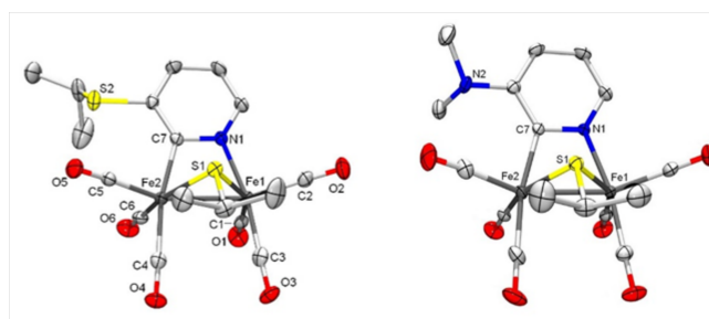
Figure 3. X-ray crystal structures of 1 (left) and 2 (right) with displacement ellipsoids drawn at 50% probability. Hydrogen atoms have been omitted for clarity. The CCDC number of 1 is 1893259 and that of 2 is 1893262. Color code: C, grey; N, blue; O, red; sulfur, yellow; iron, orange.
