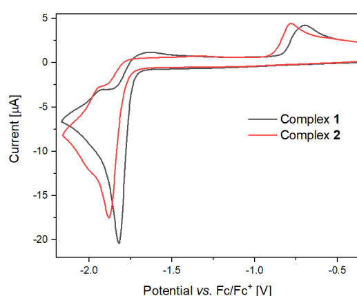
Figure 4. Cyclic voltammetry ( 0.1 \text{ V s}^{-1} ) of 1 and 2 in \text{CH}_3\text{CN} containing 0.1 \text{ M NBu}_4\text{PF}_6 on a glassy carbon working electrode.
