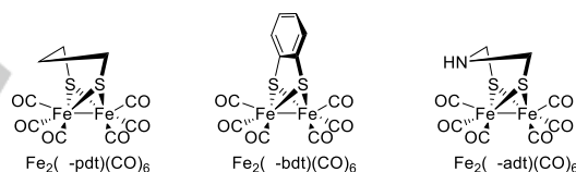
Figure 1. Common [FeFe]–H 2 ase mimics employing different dithiolate–based bridges.
