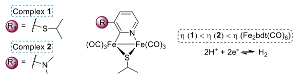
Figure 2. Structures and relative overpotentials of the novel \kappa^2\text{-C,N} pyridine di-iron complexes.
