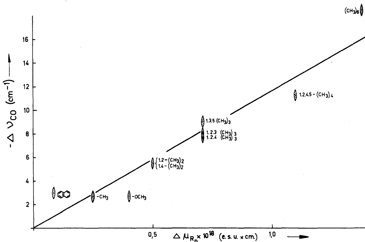
Figure 2.— E vibration mode. Plot of CO stretching frequency shifts from [\text{V}(\text{CO})_4\text{C}_6\text{H}_6]^+ vs. group moments.
