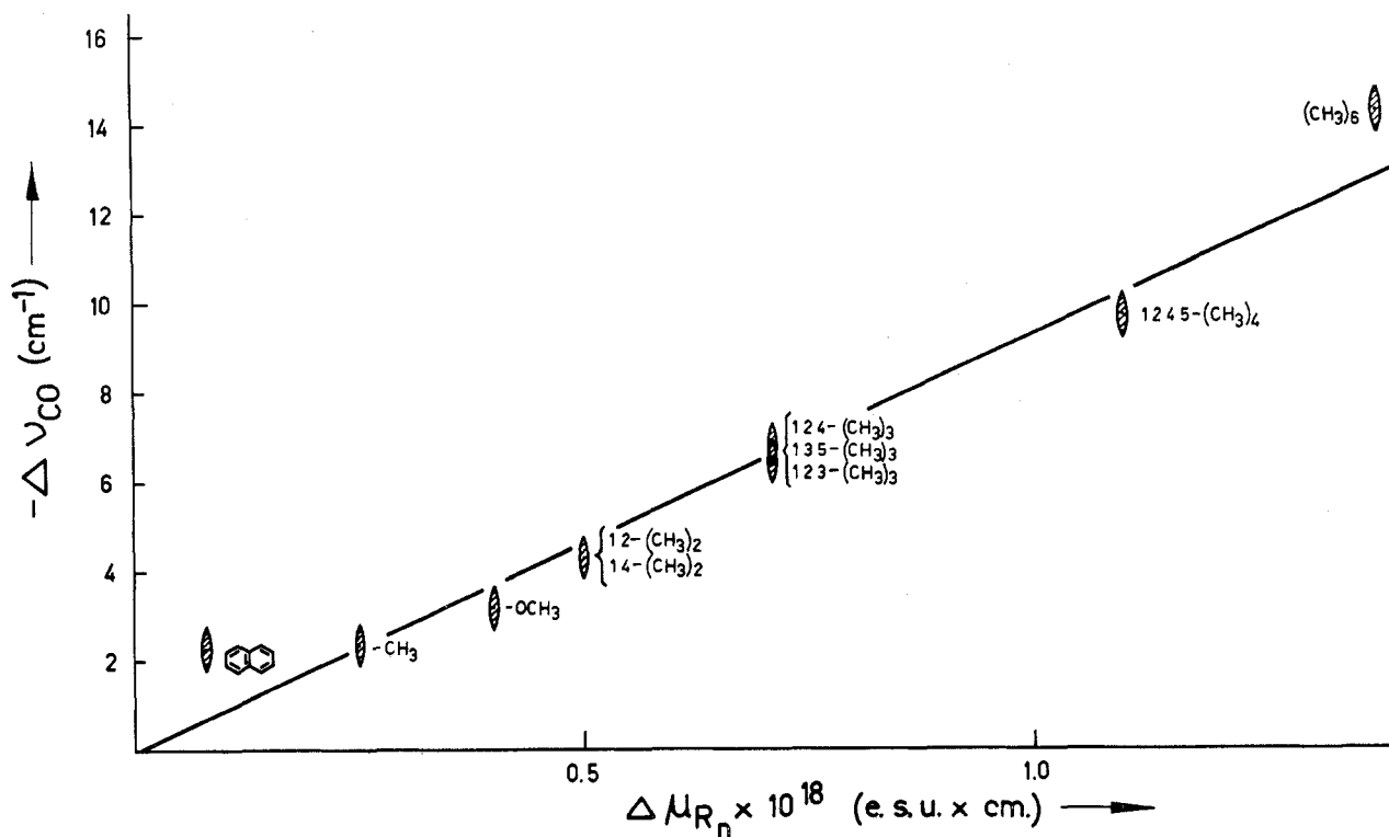
Figure 1.— A_1 vibration mode. Plot of the CO stretching frequency shifts from [\text{V}(\text{CO})_4\text{C}_6\text{H}_6]^+ vs. group moments.
