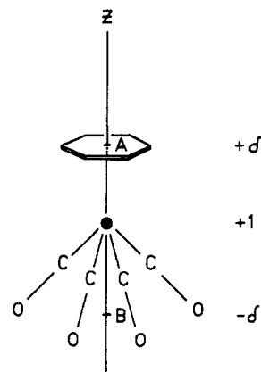
Figure 3.—Separation of partial charges in [\text{V}(\text{CO})_4\text{C}_6\text{H}_6]^+ .
