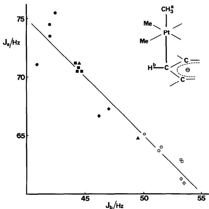
Fig. 2. Plot of values of ^2J(Pt-CH_3) against ^2J(Pt-CH) for compounds with the structural feature shown (data from this work and [5] and [9], and for the complex [PtMe_3(C_4H_3SCOCHCOCH_3)bipy] [19] for which J_a = 65.1 Hz and J_b = 50.1 Hz). Symbols refer as follows: ●, \beta -diketones [5], ■, \beta -ketoesterates; ◆, \beta -diesterates; ▲, \beta -iminoketonates [9]. Closed symbols refer to the dimers, open symbols to the adducts with the bidentate bases 2,2'-bipyridyl or 1,10-phenanthroline.
