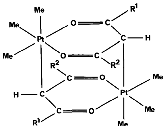
Fig. 1 Dimeric structure of the ketodiester and diester complexes of trimethylplatinum(IV). For R^1 \neq R^2 , the centrosymmetric structure with trans substituents is shown, formed from two enantiomeric monomer units ( a+b ). Two enantiomeric forms of the cis isomer ( a+a ) and ( b+b ) are also possible, the dimer now having a C_2 axis of rotation.
