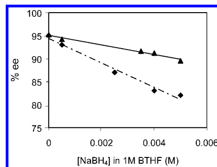
Figure 5. Addition of ▲ acetophenone or ◆ pinacolone to 1 M BTHF with increasing NaBH 4 concentrations and ( R )-MeCBS at 23 °C.
