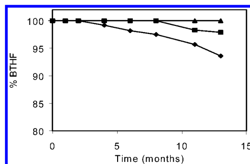
Figure 4. Shelf life of unstabilized 2 M BTHF: ◆ 2 M BTHF at 0 °C, ▲ 2 M BTHF at -20 °C, and ■ 2 M BTHF at 0 °C with 0.0035 M NaBH 4 .
