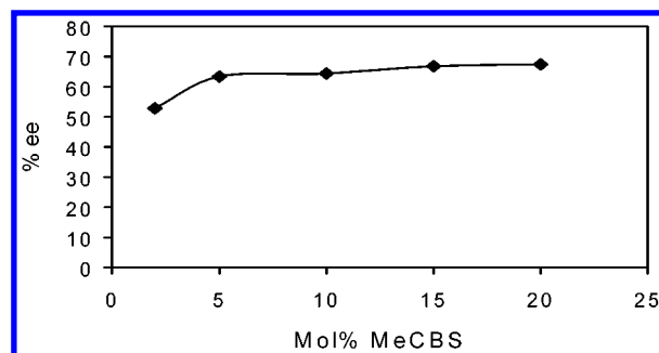
Figure 8. Effect of the catalyst concentration on % ee: commercial 1 M BTHF added to mixture of acetophenone and ( R )-MeCBS (mol % relative to ketone).
