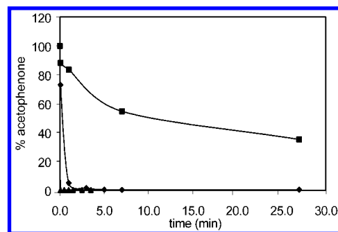
Figure 1. Reduction of acetophenone with ■ nonstabilized BTHF, ◆ NaBH 4 -stabilized BTHF, and ▲ nonstabilized BTHF and ( R )-MeCBS. The disappearance of acetophenone was monitored by GC.
