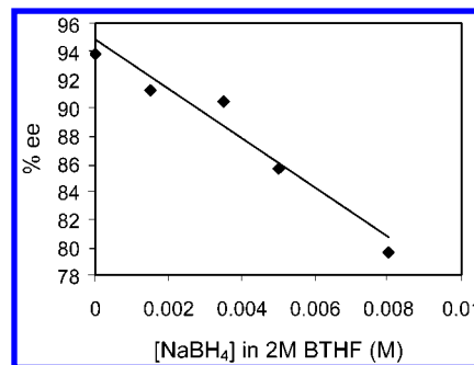
Figure 6. Addition of 2 M BTHF with increasing NaBH 4 concentrations to acetophenone and ( R )-MeCBS at 23 °C.
