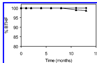
Figure 3. Shelf life of unstabilized 1 M BTHF: ▲ 1 M BTHF at 0 °C and ◆ 1 M BTHF at -20 °C.
