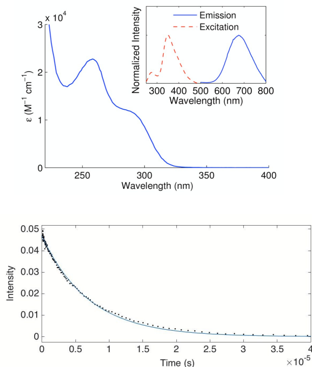
Figure 7. Top: Optical spectrum of [Cu I (SAr) 2 ]Na ( 1 ) ( I_{\text{max}} = 258 nm, \epsilon = 2.3 \times 10^4 cm -1 M -1 ); inset: excitation spectrum at 675 nm emission (dashed line) and emission spectrum at 353 nm excitation (solid line); in acetonitrile at 25 °C. Bottom: Time-resolved decay of the luminescence intensity of 1 *; in acetonitrile at 25 °C (25 mM); Xe arc lamp (425 W) at 355 nm excitation; observation wavelength: 675 nm.
