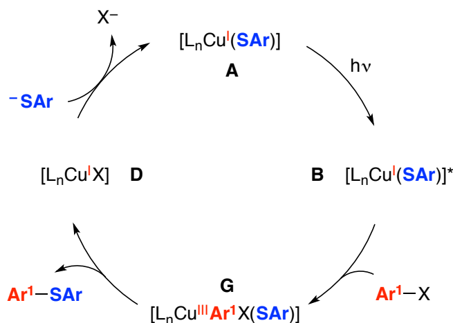
Figure 4. An alternative mechanism: Concerted oxidative addition. 5,20
