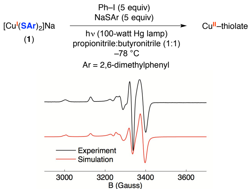
Figure 10. X-band EPR spectrum (77 K) of a coupling reaction following irradiation for 5 min. Simulation parameters: g_1 = 2.022 , g_2 = 2.032 , g_3 = 2.104 , A_1(\text{Cu}) = 85\text{ MHz} , A_2(\text{Cu}) = 130\text{ MHz} , and A_3(\text{Cu}) = 360\text{ MHz} .
