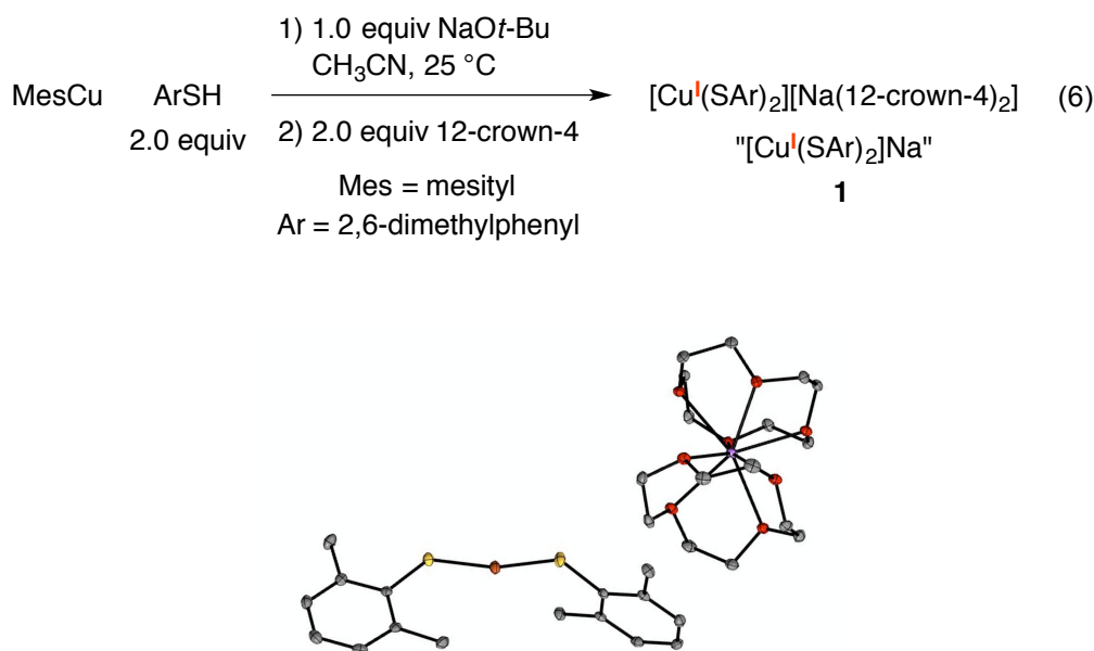
Figure 5. X-ray crystal structure of [\text{Cu}^{\text{I}}(\text{SAr})_2][\text{Na}(12\text{-crown-4})_2] ( 1 ). Ellipsoids are shown at 50% probability, and hydrogen atoms have been omitted for clarity. Selected bond lengths and bond angle: Cu–S = 2.1477(5) Å and 2.1499(5) Å; S–Cu–S, 166.82(2)°.
