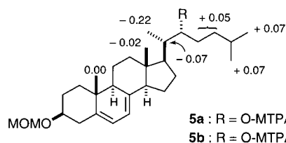
Figure 1. Distribution of \Delta\delta (= \delta S - \delta R) values (ppm, 500 MHz).
