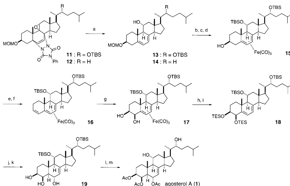
Scheme 3. Reagents and conditions: a) \text{LiAlH}_4 , \text{Et}_2\text{AlCl} , THF, 84 % from 11 , 90 % from 12 ; b) TBSOTf, 2,6-lutidine, toluene, 95 % from 13 ; c) \text{Fe}(\text{CO})_5 , 1-(4-methoxyphenyl)-4-phenyl-1-azabuta-( E , E )-1,3-diene, \text{PhCH}_3 , 94 %; d) \text{MgBr}_2 \cdot \text{Et}_2\text{O} , \text{Me}_2\text{S} , \text{CH}_2\text{Cl}_2 , 73 %; e) \text{TsCl} , Py, quant.; f) DBN, PhH, quant.; g) \text{OsO}_4 , Py, then aq. \text{NaHSO}_3 , 80 %; h) TBSOTf, DMAP, Py, quant.; i) \text{Me}_3\text{NO} , PhH, 95 %; j) \text{BH}_3\text{Me}_2\text{S} , THF, then, \text{H}_2\text{O}_2 , aq. \text{NaOH} , 62 %; k) TBAF, THF, 90 %; l) \text{Ac}_2\text{O} -Py, 91 %; m) HF-Py, THF, 84 %.
