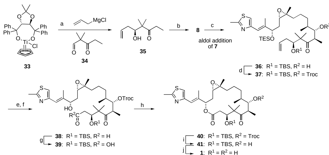
Scheme 4. a) 33 , allylmagnesium chloride, THF, 0 °C, 90 min, then add 34 , –74 °C, 3 h, 61 %; b) TBSOTf, 2,6-lutidine, CH 2 Cl 2 , –78 °C, 1 h, 87 %; c) diisopropylamine, n BuLi (1.6 M in hexanes), THF, 0 °C, 20 min, then add 8 (in THF), –78 °C to –40 °C, 30 min, then add 7 (in THF), –78 °C, 15 min, 92 %; d) TrocCl, CH 2 Cl 2 , pyridine, 20 °C, 30 min, 91 %; e) NMO, OsO 4 (5 mol %), THF/ t BuOH/H 2 O 10:10:1, 25 °C, 16 h, workup with Na 2 S 2 O 3 ; crude diol in EtOH/H 2 O, NaIO 4 , 25 °C, 1 h, 78 % over two steps; f) HF/pyridine, THF, 22 °C, 20 min, 91 %; g) NaClO 2 , 2,3-dimethyl-2-butene, NaH 2 PO 4 , t BuOH, H 2 O, 22 °C, 45 min, 92 %; h) 38 , 2,4,6-trichlorobenzoyl chloride, triethylamine, DMAP, 0.02 M solution in toluene, 22 °C, 90 min, 65 %; i) Zn, ammonium chloride, EtOH, reflux, 20 min, 92 %; j) HF/pyridine, 35 °C, 7d , 67 %. Tf = trifluoromethanesulfonyl; TrocCl = 2,2,2-trichloroethyl chloroformate; DMAP = 4-dimethylaminopyridine.
