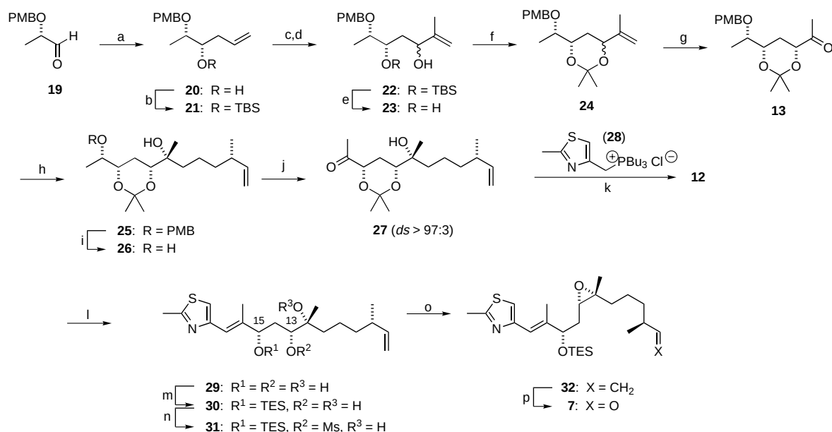
Scheme 3. a) See ref. [11]; b) TBSCl, imidazole, DMF, 22 °C, 24 h, 97 %; c) O 3 , CH 2 Cl 2 /MeOH, –78 °C, then PPh 3 , 98 %; d) isopropenyl magnesium bromide, THF, –10 °C, 45 min, 89 % as a 3:2-mixture of diastereomers; e) 1.2 equiv TBAF, THF, 1 h, 25 °C, 99 %; f) 2,2-dimethoxypropane, cat. TsOH, 99 %; g) O 3 /PPh 3 , CH 2 Cl 2 , –78 °C, then 2.0 equiv K 2 CO 3 , MeOH, 1 h, 25 °C, (94 % in two steps); h) MgBr 2 , CH 2 Cl 2 , –78 °C, 3.0 equiv 14 , 3 h, (78 %, ds = 96:4); i) 1.2 equiv DDO, CH 2 Cl 2 , 45 min, 25 °C, (98 %); j) 1.5 equiv Dess–Martin-periodinane, CH 2 Cl 2 , 2 h, 25 °C, 95 %; k) 5.0 equiv 28 , KHMDS, 0 °C, 40 min, then 27 , 45 °C, 20 min, THF, 80 %; l) 15 % HCl, MeOH, 12 h, 25 °C, 99 %; m) 3.0 equiv TESCl, Et 3 N, CH 2 Cl 2 , 12 h, 25 °C, 90 %; n) MsCl, Et 3 N, 92 %; o) K 2 CO 3 , MeOH, 1 h, 25 °C, 90 %; p) NMO, OsO 4 , NaIO 4 , (62 % in two steps). TBS = tert -butyldimethylsilyl; TBAF = tetrabutylammonium fluoride; Ts = 4-toluenesulfonyl; DDO = 2,3-dichloro-3,4-dicyanobenzoquinone; KHMDS = potassium hexamethyldisilazide; TES = triethylsilyl; Ms = methanesulfonyl, NMO = 4-methylmorpholine- N -oxide.
