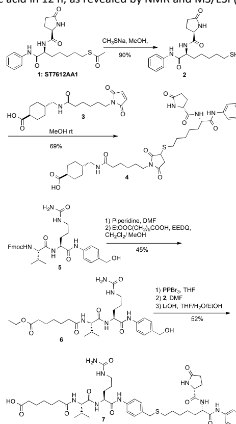
Scheme 1 Preparation of payloads/linkers for conjugation.
