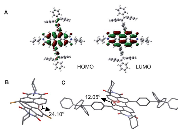
Fig. 3 (A) Molecular orbital amplitude plots of HOMO and LUMO energy levels of 1,7-DTPEPBI. (B) and (C) show the optimal structures of 1,7-DBrPBI and 1,7-DTPEPBI calculated by the semi-empirical AM1 method. The white, grey, blue, red, and scarlet balls represent H, C, N, O, and Br atoms, respectively. The H atoms are omitted for clarity.
