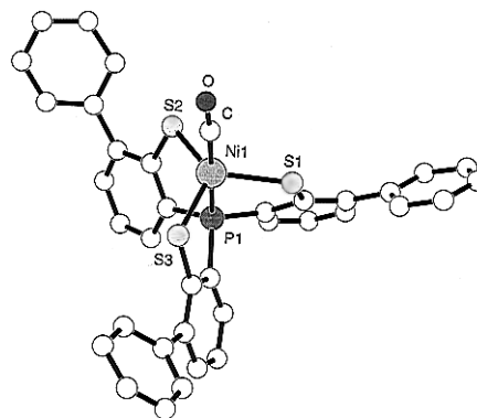
Figure 1. Structural diagram of [Ni(PS3*)(CO)] 1− . Selected bond distances (Å) and angles (deg): Ni–S1, 2.352(6); Ni–S2, 2.274(5); Ni–S3, 2.312(6); Ni–C37, 1.75(3); Ni–P1, 2.089(6); C37–O1, 1.15(2); S1–Ni–S2, 122.6(2); S1–Ni–S3, 109.8(2); S2–Ni–S3, 124.2(2); S1–Ni–P1, 82.6(2); S2–Ni–P1, 83.8(2); S3–Ni–P1, 85.1(2); S1–Ni–C37, 98.1(9); S2–Ni–C37, 92.8(8); S3–Ni–C37, 97.9(8); P1–Ni–C37, 176.4(8).
