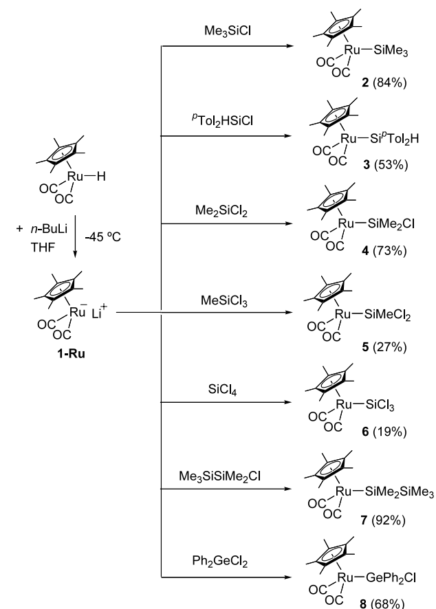
Scheme 2. Generation and reactions of \text{Li}[(\eta^5\text{-C}_5\text{Me}_5)\text{Ru}(\text{CO})_2] ( 1-Ru ).
