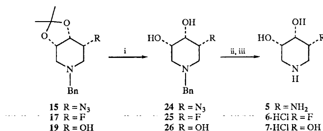
Scheme 4 Reagents and conditions: i, TFA–water (4:1), room temp., 2 h; ii, H 2 (3 atm), 10% Pd–C, MeOH, 40 °C, 1 h; iii, 1 mol dm −3 HCl (2 mol equiv.), MeOH (for 6 ·HCl and 7 ·HCl)
