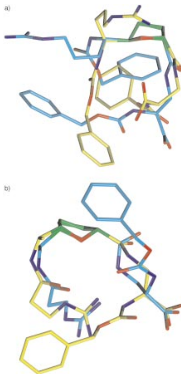
Figure 13. Overlay of low energy conformations of THF-based RGD mimetics, THF ring in green; top: 40 (yellow 83 % and blue 15 % populated at 298 K); bottom: 62 (yellow 87 % and blue 8 % populated at 298 K).
