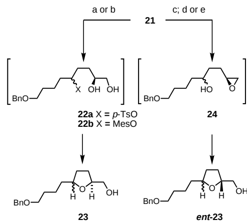
Scheme 2. Stereocomplementary routes to the THF alcohols 23 and ent-23 : a) i) p -TsCl, pyridine, CH 2 Cl 2 , rt, 2 h; ii) HOAc, H 2 O, rt, 13 h; iii) NaH, THF/DMSO, 40 °C, 4 h, 63% from 21 ; b) i) MesCl, Et 3 N, CH 2 Cl 2 , −15 °C, 1 h; ii) 1N HCl, THF, rt, 2 h, 77% from 21 ; c) 1N HCl, THF, rt, 2 h, 90%; d) i) mesitylenesulfonyl chloride, pyridine, CH 2 Cl 2 , 0 °C, 36 h; ii) K 2 CO 3 , MeOH, rt, 2 h; iii) HOAc, CH 2 Cl 2 , rt, 2 h, 48%; e) NaH, tosylimidazole, THF, rt, 45 min, 77%. p -Ts = para -toluenesulfonyl, Mes = methanesulfonyl, DMSO = dimethyl sulfoxide.
