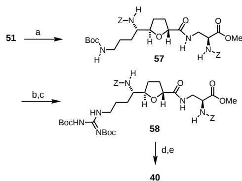
Scheme 7. Synthesis of the RGD-mimetic 40 : a) 27 , HOBt, EDC, \text{EtN}(i\text{Pr})_2 , THF, rt, 16 h, crystallization of the trans isomer, 37%; b) TFA, \text{CH}_2\text{Cl}_2 , rt, 2 h; c) 54 , \text{HgCl}_2 , \text{Et}_3\text{N} , DMF, rt, 3 h, 73% from 57 ; d) i) LiOH, THF, \text{H}_2\text{O} , rt, 20 min; ii) TFA, \text{CH}_2\text{Cl}_2 , rt, 2 h, 46% from 58 .
