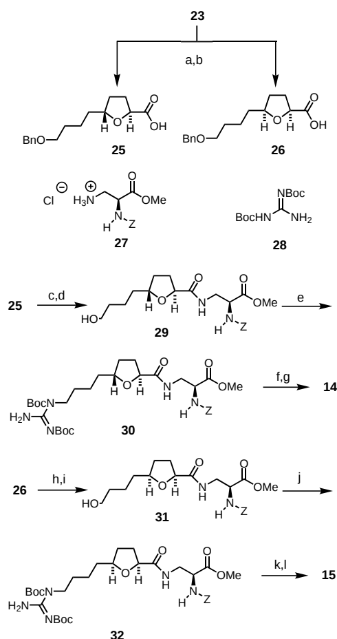
Scheme 3. Synthesis of the RGD-mimetics 14 and 15 : a) (COCl) 2 , DMSO, Et 3 N, CH 2 Cl 2 , −60 → 0 °C, 30 min; b) NaClO 2 , NaH 2 PO 4 , amylene, t -BuOH, rt, 12 h, 77%; 40% of 25 and 21% of 26 after chromatography; c) H 2 , 10% Pd/C, THF/MeOH/H 2 O 4:2:1, rt, 18 h; d) 27 , BOP, EtN( i Pr) 2 , MeCN, rt, 16 h, 89% from 25 ; e) 28 , PPh 3 , diisopropyl azodicarboxylate, THF, rt, 16 h, 62%; f) LiOH, THF, H 2 O, rt, 20 min; g) TFA, CH 2 Cl 2 , rt, 2 h, 85% from 30 ; h) and i) see c) and d), 62% from 26 ; j) see e), 74%; k) and l) see f) and g), 79% from 32 . BOP = 1-benzotriazol-1-yloxytris(dimethylamino)phosphonium hexafluorophosphate, TFA = trifluoroacetic acid.
