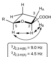
Figure 7. Stereochemical assignment of the cis configuration of 26 from NMR data.
