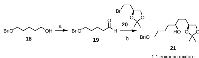
Scheme 1. Preparation of the alcohol 21 : a) (COCl) 2 , DMSO, Et 3 N, CH 2 Cl 2 , −60 → 0 °C, 30 min, 98%; b) Mg, THF, 0 °C, 20 min, 80%.
