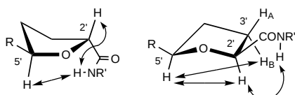
Figure 11. Stereocenter assignment of the relative configuration at the THF rings of 38 , 39 , and 40 from NOESY data.
