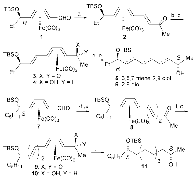
Scheme 2 Reagents and conditions: (a) \text{CH}_3\text{COCH}_2\text{P}(\text{OMe})_2 , \text{LiOH} \cdot \text{H}_2\text{O} , \text{MeOH} (90% for 1 , 78% for 7 ); (b) NaH, THF (81%), (c) \text{NaBH}_4 , \text{MeOH} (91% for 3 , 72% for 8 ); (d) \text{H}_2\text{O}_2 , 1 M NaOH, \text{MeOH} , 0 °C (83%); (e) \text{H}_2 , \text{PtO}_2 , \text{AcOEt} (85%); (f) (\text{EtO})_2\text{P}(\text{O})\text{CH}_2\text{CN} , NaH, THF, 0 °C (69%); (g) DIBAL-H, -50 °C (49%); (h) n\text{-Bu}_3\text{P} , \text{CH}_2\text{Cl}_2 (71%); (i) \text{KN}(\text{SiMe}_3)_2 , THF, 0 °C (70%); (j) \text{H}_2\text{O}_2 , 1 M NaOH; \text{H}_2 , \text{PtO}_2 (89%).
