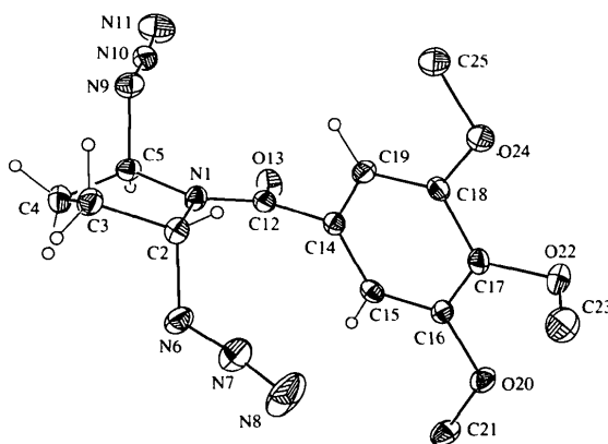
Fig. 2. Displacement ellipsoid plot of (II) showing the atom-labeling scheme; ellipsoids are scaled to the 30% probability level. H atoms are represented as spheres of arbitrary radii.
