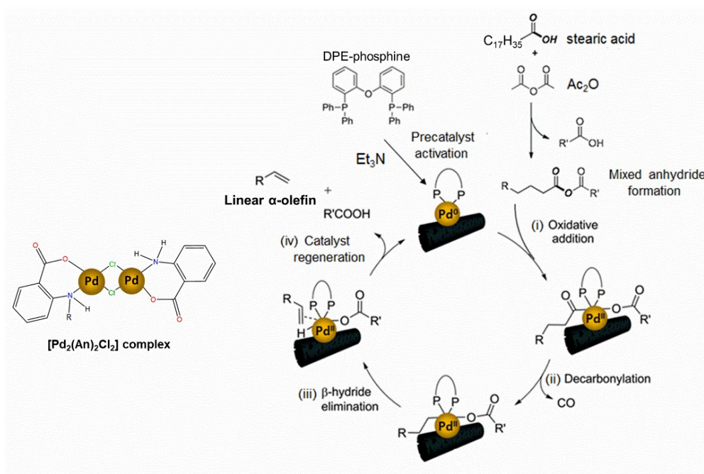
Scheme 6 Possible reaction mechanism of the AnPd/CNF-catalyzed decarbonylation of stearic acid to linear \alpha -olefins. (Scheme adapted) 14, 58
