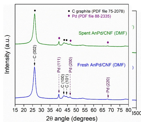
Fig. 12 Powder XRD patterns of the AnPd/CNF (DMF) catalyst before and after decarbonylation reaction
