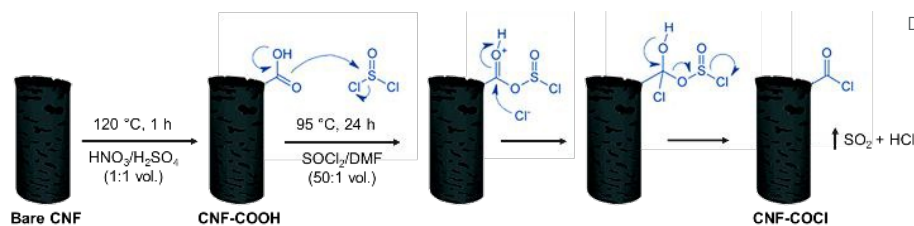
Scheme 1 Surface acyl chlorination of the carbon nanofibers support. (Scheme adapted) 37
