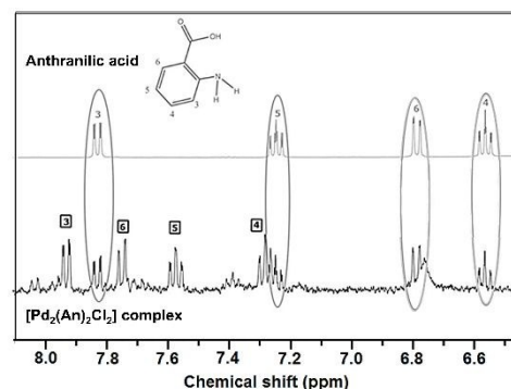
Fig. 1 1 H NMR spectra of the expanded view of the aromatic region of anthranilic acid and the [Pd 2 (An) 2 Cl 2 ] complex performed in acetone- d 6 .
