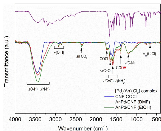
Fig. 8 FTIR spectra of the synthesized materials.
