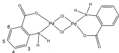
Scheme 3 Suggested chemical structure of the synthesized di-μ-chloro-Bis[palladium(II) anthranilate] ([Pd 2 (An) 2 Cl 2 ]) complex. Numerical scheme for 1 H NMR spectroscopic studies.
