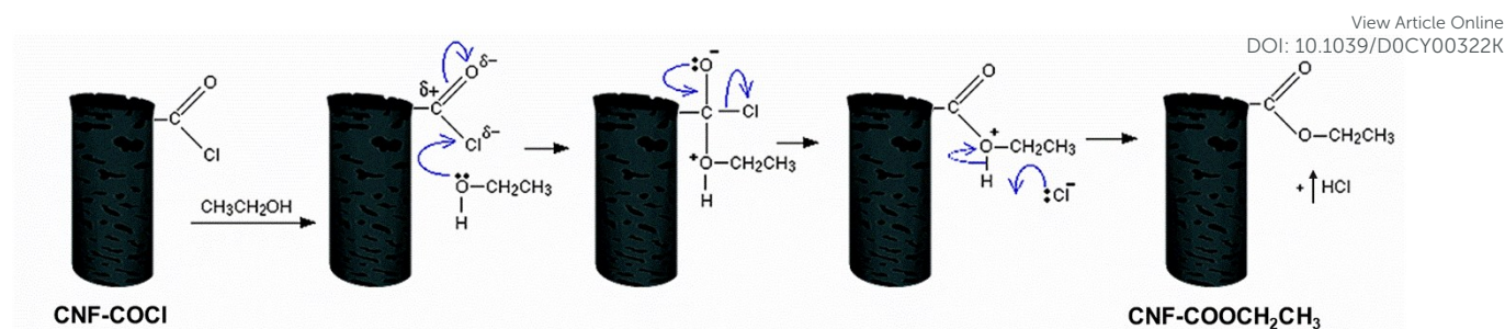
Scheme 5 Blocking of the acyl chloride groups by nucleophilic addition/elimination reaction with EtOH.
