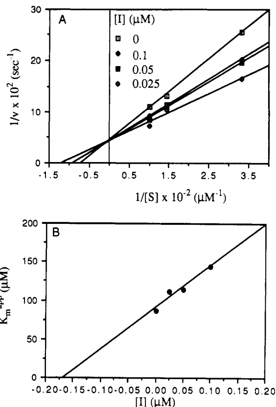
Figure 2. Competitive inhibition assay of α-chymotrypsin with the iodo enol lactone 4: panel A, determination of K_m^{app} at different inhibitor concentrations; panel B, A plot of K_m^{app} versus [I] gives a straight line with an x-intercept of -K_i .
