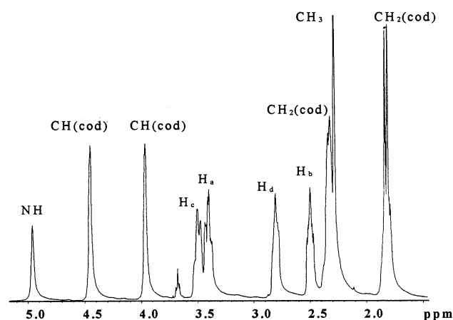
Fig. 2. ^1H -NMR of [Rh(cod)(N\text{-methylpiperazine})]CF_3SO_3 .
