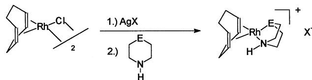
Scheme 5. Preparation of cationic [Rh(cod)(amine)]^+ complexes with bidentate amines.
