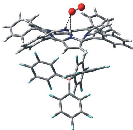
Fig. 4 DFT/M05-2x optimized structure of \{(H_4TPP^{2+})-(TB^-)-O_2\} system; the averaged O–H distances were calculated to be 2.338 Å.
