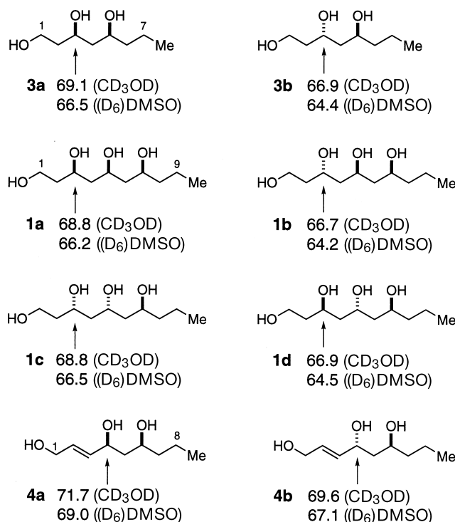
Fig. 4. ^{13}\text{C} -NMR Chemical shifts (ppm; in (\text{D}_6)\text{DMSO} and \text{CD}_3\text{OD} ) of C(3) of 1a – d and 3a,b , and of C(4) of the olefinic 1,3-diols 4a and 4b
