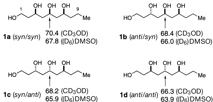
Fig. 1. ^{13}\text{C} -NMR Chemical shifts (ppm; in (\text{D}_6)\text{DMSO} and \text{CD}_3\text{OD} ) of C(5) of 1a–d
