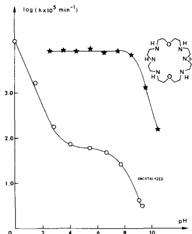
Fig. 4. pH-Dependence of the rate of ATP-hydrolysis catalyzed by macrocycle 1 and uncatalyzed. Plot of \log(k_{\text{obs}} \times 10^5 \text{ min}^{-1}) vs. pH for: (★) the hydrolysis of 0.03M ATP macrocyclic polyamine 1 at 60° in \text{D}_2\text{O}/\text{H}_2\text{O} 1:9; (○) the uncatalyzed rate of hydrolysis at 70° reported in [21].
