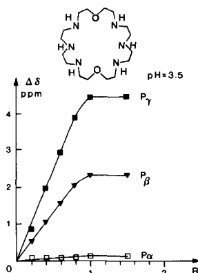
Fig. 2. ^{31}\text{P} -NMR shifts ( |\Delta\delta| ) of the \alpha -, \beta - and \gamma -phosphate signals of ATP as a function of increasing ligand/substrate ratio R = L/S = 1/ATP at pH = 3.5 ( \text{D}_2\text{O}/\text{H}_2\text{O} 1 : 9 solution, 0.03M ATP; 20^\circ )
