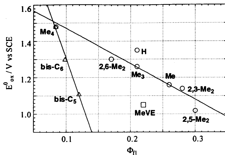
Fig. 4. Correlation between quantum yield of fluorescence and oxidation potential of sensitizers. E_{\text{ox}}^0 = -10.13 \times \Phi_{\text{fl}} + 2.32 , r = 0.994 . E_{\text{ox}}^0 = -1.95 \times \Phi_{\text{fl}} + 1.67 , r = 0.946 .
