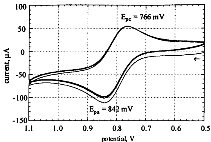
Fig. 2. Cyclic voltammogram of 3.33 mM MeVE in MeCN containing 0.1M \text{Bu}_4\text{N}^+\text{PF}_6^- at a sweep rate of 100 mV/s vs \text{Ag}^+/\text{AgNO}_3 . E_{1/2} = 1.054 V vs. SCE. E_p^a - E_p^c = 76 mV.
