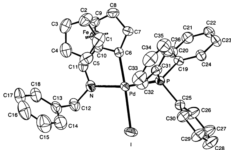
Fig. 3. Molecular structure and atom labelling scheme for [Pd{[(η 5 -C 5 H 3 )-CH=N-CH 2 -C 6 H 5 ]Fe(η 5 -C 5 H 5 )}(I)(PPh 3 )].
