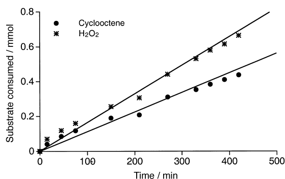
Figure 6. Reaction profile for the oxidation of cyclooctene. Reaction conditions: substrate (1 mmol), catalyst (0.01 mmol), 1,2-dichloroethane (1 mL), 35 % \text{H}_2\text{O}_2 (3 mmol), T = 60^\circ\text{C} . Cyclooctene consumption was determined by GC, \text{H}_2\text{O}_2 consumption was determined from the amount used to form cyclooctene oxide and the amount of oxygen formed (gas burette). k_{\text{co}} = 1.16 \text{ mmol min}^{-1} , k_{\text{H}_2\text{O}_2} = 1.64 \text{ mmol min}^{-1} .
