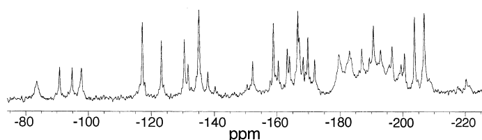
Figure 5. ^{183}\text{W} NMR spectrum of \text{Li}_9[\text{Ni}(\text{H}_2\text{O})\text{H}_2\text{F}_6\text{NaW}_{17}\text{O}_{55}] in \text{D}_2\text{O} .
