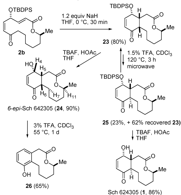
Scheme 5. Preparation of Sch 642305 ( 1 )
