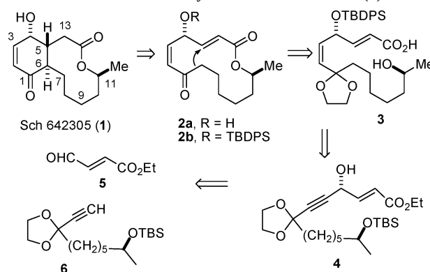
Scheme 1. Retrosynthesis of Sch 642305 ( 1 )
