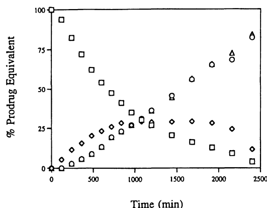
Fig. 2. Stability of cyclic prodrug 2 at 37°C in HBSS buffer, pH 7.4, showing the time course of disappearance of the cyclic prodrug (□) and the appearance of the intermediate (◇), DADLE (○) and coumarin (Δ).
