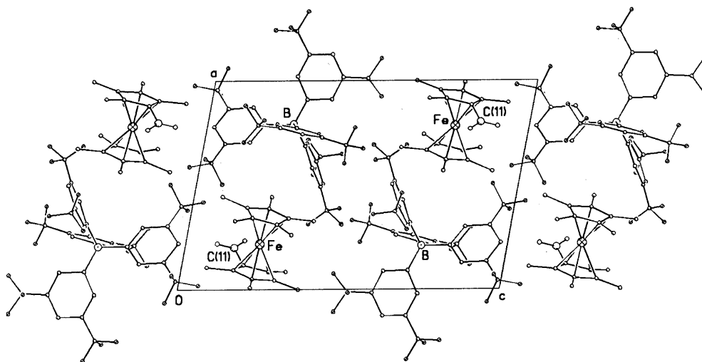
Fig. 2. Fragment of crystal packing of 1\mathbf{a} \cdot \text{B}\{\text{C}_6\text{H}_3(\text{CF}_3)_2-3,5\}_4 projection onto the (010) crystallographic plane.
