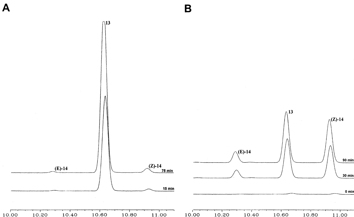
Fig. 1. The hydrosilylation of cyclopropyl phenyl ketone catalyzed by complex 1 (chromatogram A) and complex 2 (chromatogram B), respectively. Both chromatograms show ca. 20% of the catalyzed reaction.
