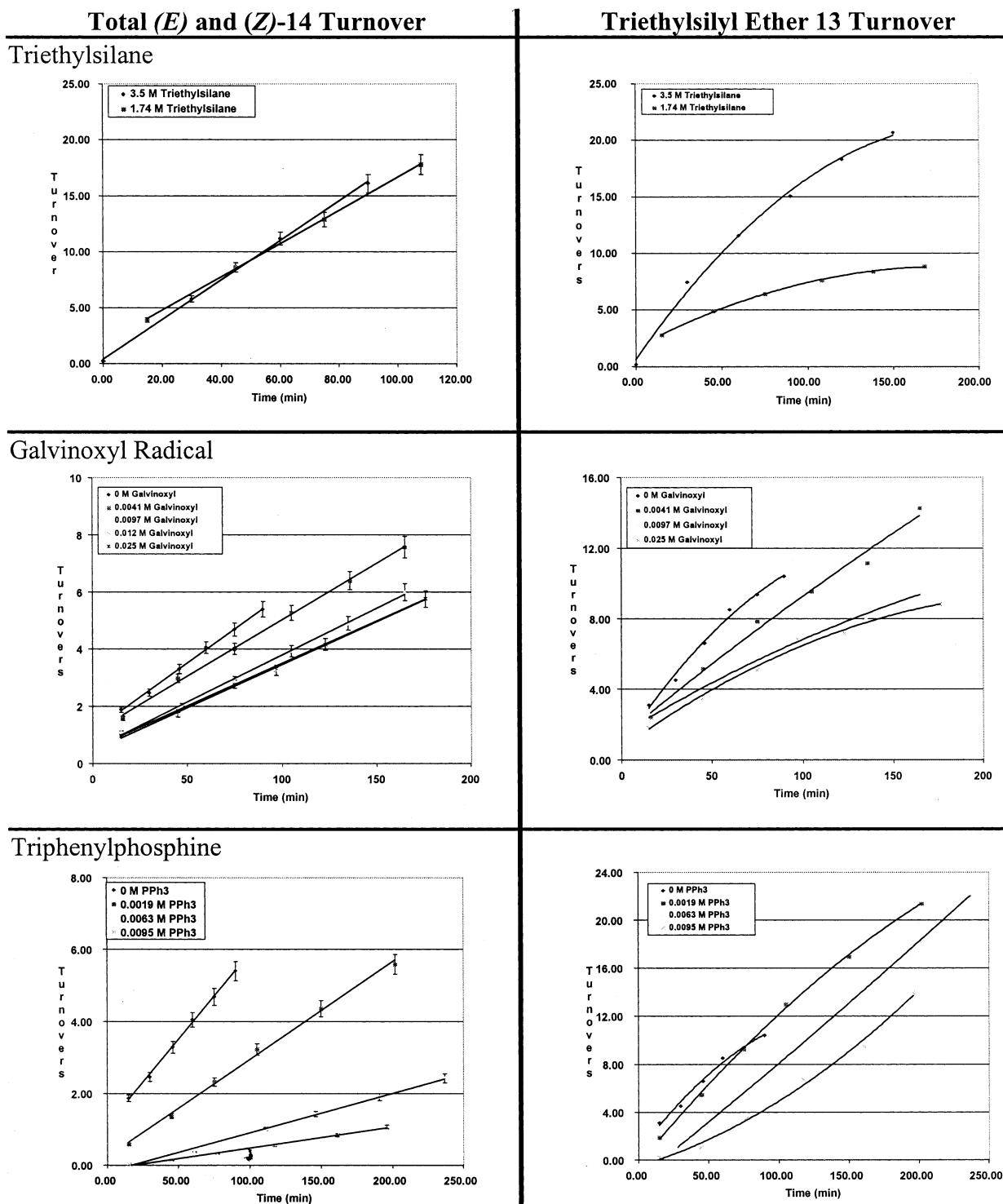
Fig. 2. Initial turnover rate studies for the reaction of ketone 9 with triethylsilane catalyzed by complex 2 . The reaction additive is highlighted for each set of experiments.
