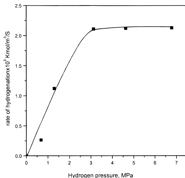
Figure 1. Effect of hydrogen pressure on initial rate of hydrogenation of nitrobenzene to p -aminophenol. Reaction conditions: nitrobenzene, 1.86 \text{kmol}/\text{m}^3 ; catalyst, 0.35 \text{kg}/\text{m}^3 ; water, 70 \times 10^{-6} \text{ m}^3 ; acid, 10% w/w; temperature, 353 K; agitation, 700 rpm; total reaction volume, 1 \times 10^{-4} \text{ m}^3 .
