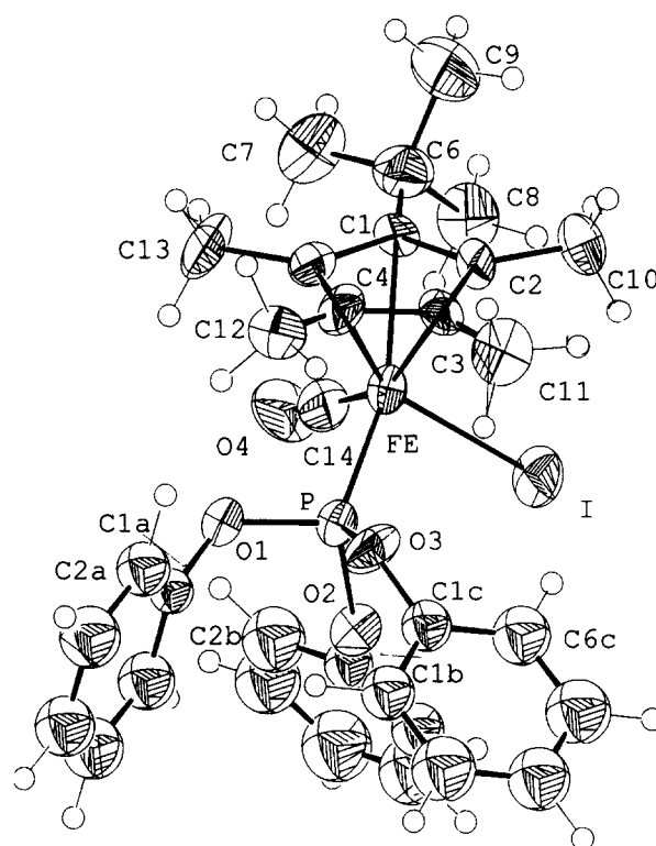
Fig. 3. ORTEP plot of 2 (side view).
