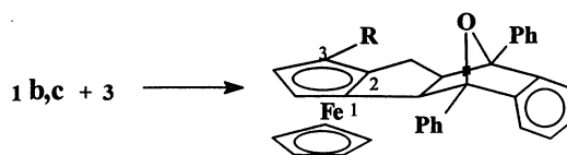
16a,b ( R = ^t\text{Bu-} ) and 17a,b ( R = ^1\text{Ad-} )
