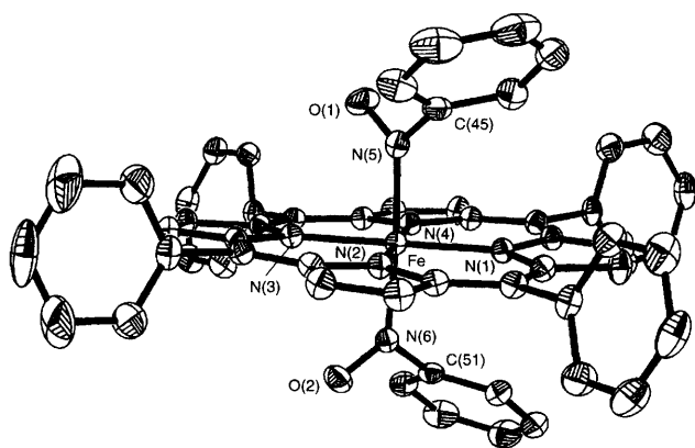
Fig. 1 Molecular structure of 1 . Hydrogen atoms have been omitted for clarity. Selected bond distances ( \text{\AA} ) and angles ( ^\circ ): Fe–N(1) 2.003(2) , Fe–N(2) 1.994(2) , Fe–N(3) 1.995(2) , Fe–N(4) 1.998(2) , Fe–N(5) 1.874(2) , N(5)–O(1) 1.237(3) , Fe–N(6) 1.899(2) , N(6)–O(2) 1.227(3) ; Fe–N(5)–O(1) 123.6(2) , Fe–N(6)–O(2) 123.4(2) .
