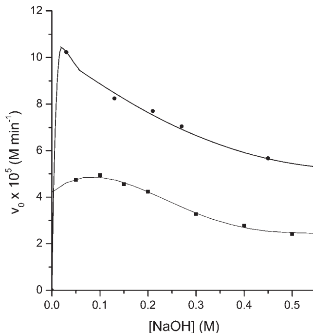
Figure 3. Variation of v_0 with respect to [\text{NaOH}] . [\text{Fe}(\text{CN})_6^{3-}]_0 = 8.0 \times 10^{-3} \text{ M} , [\text{2,3-butanediol}]_0 = 0.02 \text{ M} , [\text{Ru}]_0 = 1.0 \times 10^{-6} \text{ M} , I = 0.5 \text{ M} and T = 30^\circ\text{C} . Ru(III) (a) and Ru(VI) (b).
