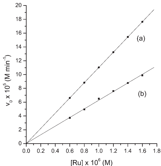
Figure 2. Effect of [\text{catalyst}]_0 on the initial rate. [\text{2,3-butanediol}]_0 = 0.05 \text{ M} , [\text{Fe}(\text{CN})_6^{3-}]_0 = 8.0 \times 10^{-4} \text{ M} , [\text{OH}^-] = 0.15 \text{ M} , T = 30^\circ\text{C} , I = 0.5 \text{ M} . Ru(III) (a) and Ru(VI) (b).
