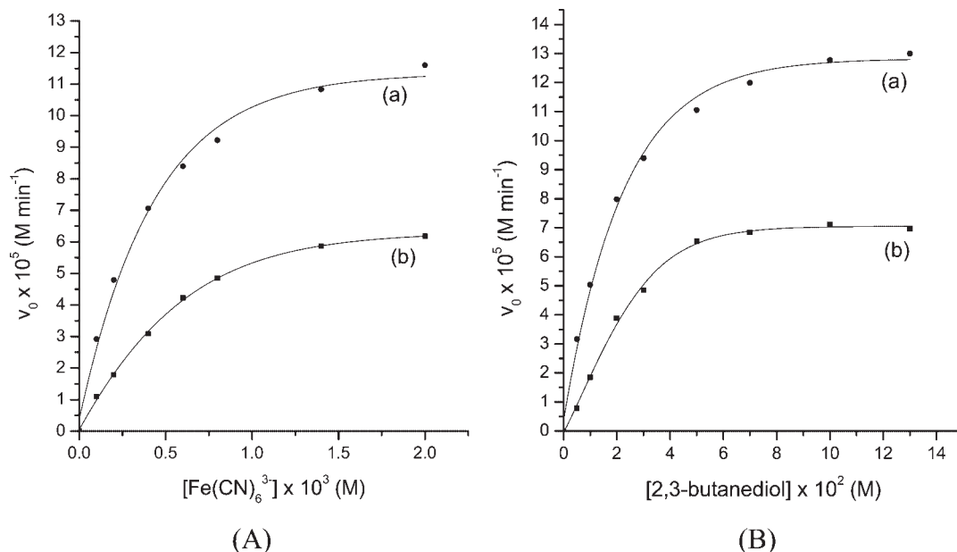
Figure 1. Plots of v_0 versus [\text{Fe}(\text{CN})_6^{3-}]_0 , [\text{2,3butanediol}] = 0.03 \text{ M} (A) and plots of v_0 versus [\text{2,3-butanediol}]_0 , [\text{Fe}(\text{CN})_6^{3-}]_0 = 8.0 \times 10^{-4} \text{ M} (B). [\text{Ru}]_0 = 1.0 \times 10^{-6} \text{ M} , [\text{NaOH}] = 0.15 \text{ M} , I = 0.5 \text{ M} and T = 30^\circ \text{C} . Ru(III) (a) and Ru(VI) (b).
