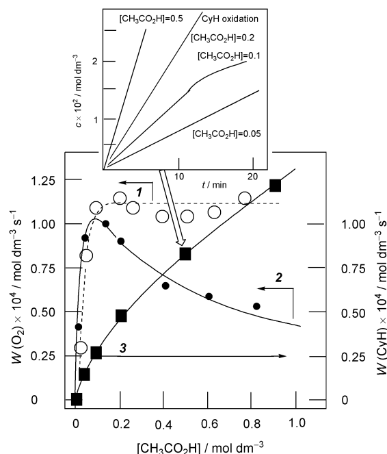
Fig. 2 Decomposition of H 2 O 2 (0.25 mol dm −3 ) catalysed by complex 1a (5 × 10 −5 mol dm −3 ). The dependence of the O 2 evolution rate on [CH 3 CO 2 H] in the absence (curve 1) and in the presence (curve 2) of cyclohexane (0.46 mol dm −3 ), as well as the analogous dependence for the initial rate of cyclohexanol and cyclohexanone (after PPh 3 reduction) accumulation (curve 3) are shown. Curves of oxygenate accumulation with time in the cyclohexane oxidation at various acetic acid concentrations are shown in the inset at the top of the figure. Initial rates of these reactions are plotted as curve 3 in the main graph.
