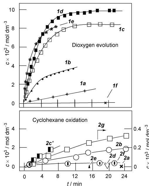
Fig. 1 Decomposition of H 2 O 2 (0.25 mol dm −3 ) in the presence of cyclohexane (0.46 mol dm −3 ) and cyclohexane oxidation catalysed by complex 1a (5 × 10 −5 mol dm −3 ). Kinetic curves are presented for the O 2 evolution (1) and for the sum of cyclohexanol and cyclohexanone (after PPh 3 reduction) accumulation (2) in the absence of any additive (curves a) and in the presence of acetic acid ([CH 3 CO 2 H] = 0.05 mol dm −3 ) (curves b), in the presence simultaneously of acetic acid ([CH 3 CO 2 H] = 0.05 mol dm −3 ) and of n -Bu 4 NOH at various concentrations: 10 × 10 −5 (curves c) {at [H 2 O 2 ] 0 = 0.75 mol dm −3 (curve c'), 20 × 10 −5 mol dm −3 (curves d), or of TMTACN (10 × 10 −5 mol dm −3 ) (curves e), as well as in the presence of HClO 4 (10 × 10 −5 mol dm −3 ) (curves f) and simultaneously CH 3 CO 2 H (0.05 mol dm −3 ) and HClO 4 (5 × 10 −5 mol dm −3 ) (curve g).
