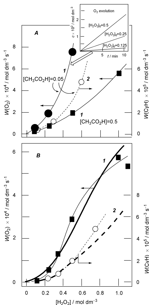
Fig. 5 Dependence of the \text{O}_2 evolution rate (curves 1) and the cyclohexane oxygenation rate (curves 2) on initial concentration of hydrogen peroxide. Graph A: \text{CH}_3\text{CO}_2\text{H} (0.05 or 0.5 \text{mol dm}^{-3} ), 1a ( 5 \times 10^{-5} \text{mol dm}^{-3} ). Graph B: \text{CH}_3\text{CO}_2\text{H} (0.05 \text{mol dm}^{-3} ), 1a ( 1 \times 10^{-5} \text{mol dm}^{-3} ), n\text{-Bu}_4\text{NOH} ( 4 \times 10^{-5} \text{mol dm}^{-3} ) and (for curve 2) cyclohexane (0.46 \text{mol dm}^{-3} ). On graph B bold curves for the \text{O}_2 evolution (curve 1) and for the cyclohexane oxygenation (curve 2) were simulated using eqns. (1)–(7) and the conditions in eqns. (8)–(11). Curves of dioxygen evolution and oxygenate accumulation with time in the hydrogen peroxide decomposition at various hydrogen peroxide concentrations are shown in the inset at the top of the figure. Initial rates of these reactions are plotted as curve 1 in graph A.
