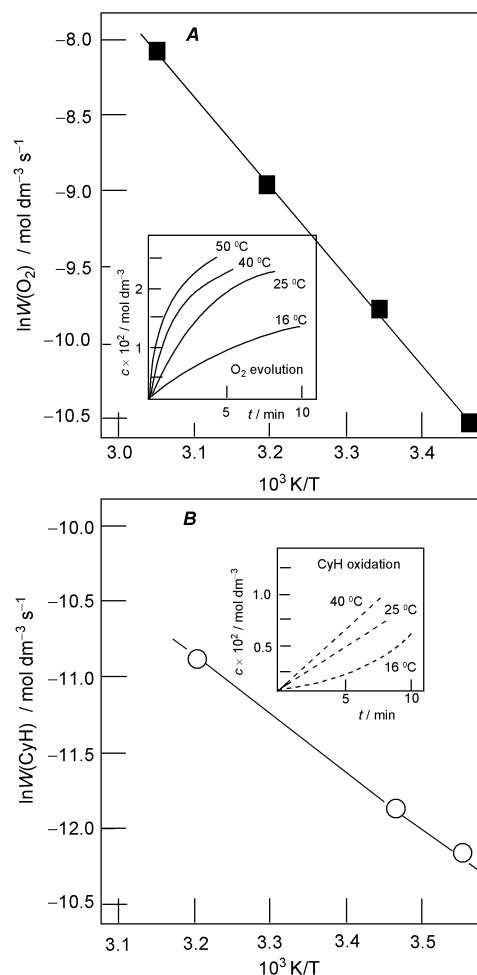
Fig. 6 Dependence of the \text{O}_2 evolution rate W(\text{O}_2) (graph A) and the cyclohexane oxygenation rate W(\text{CyH}) (graph B) on temperature. Conditions: cyclohexane (0.46 \text{mol dm}^{-3} ), 1a ( 5 \times 10^{-5} \text{mol dm}^{-3} ), \text{H}_2\text{O}_2 (0.25 \text{mol dm}^{-3} ), \text{CH}_3\text{CO}_2\text{H} (0.05 \text{mol dm}^{-3} ). Curves of dioxygen evolution and oxygenate accumulation with time at various temperatures are shown in the insets. Initial rates of these reactions are plotted in the main graphs.
