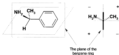
Fig. 1. The quadrant projection of ( S )-(1-phenylethyl)amine (according to Smith and co-workers [10–12]). ‘The sequences for the summation of contributions to the 1 L b CEs (given by Smith and Fontana [10]) are SH, COO – , Me 3 C > Me, CH 2 > NH 2 , + NH 3 , Me 3 N + , OH, MeO, Cl; and Me > COOH > + NH 3 , OH, MeO. These sequences may be used in connection with the sector signs in quadrant projection and will have a general usefulness for the establishment of the absolute configuration of related chiral benzene compounds in which one substituent at the contiguous chiral center is a hydrogen atom’.
