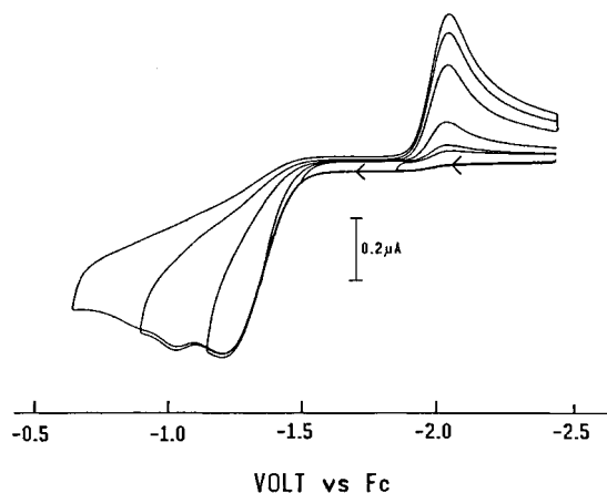
Figure 6. CV scans of 1_2^{2-} in THF/0.1 M [NBu 4 ][PF 6 ] ( \nu = 0.5 \text{ V s}^{-1} ) from -2.45 \text{ V} to increasingly positive potentials at 252 K. 1_2^{2-} was prepared from bulk electrolytic reduction of a solution of 1 at E_{\text{appl}} = -2.3 \text{ V} .
