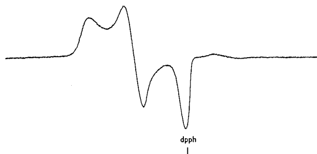
Figure 3. ESR spectrum at 77 K of 1^+ in 1/1 \text{CH}_2\text{Cl}_2/\text{C}_2\text{H}_4\text{-Cl}_2 produced by reaction of 1 with equimolar [(p\text{-BrC}_6\text{H}_4)_3\text{N}]^+ .
