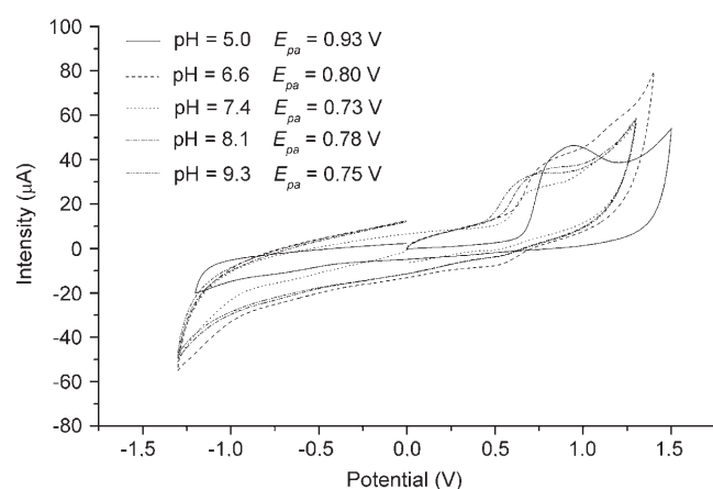
Figure 1. Cyclic voltammograms of the free ligand EDDHA ( 1\text{ mM} ) in 0.1\text{ M} buffered phosphate solutions.
