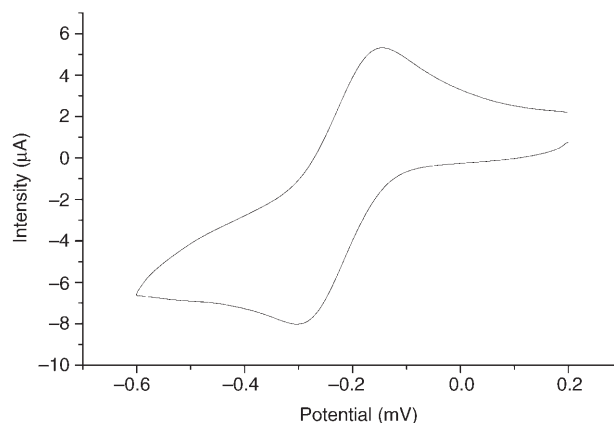
Figure 4. Cyclic voltammogram of \text{Fe}^{\text{III}}-o,p\text{-EDDHA} . Conditions: [\text{FeCl}_3 \cdot 6\text{H}_2\text{O}] 10^{-3} M, [o,p\text{-EDDHA}] 10^{-2} M in 0.1 M buffered phosphate solution, at pH 5.
