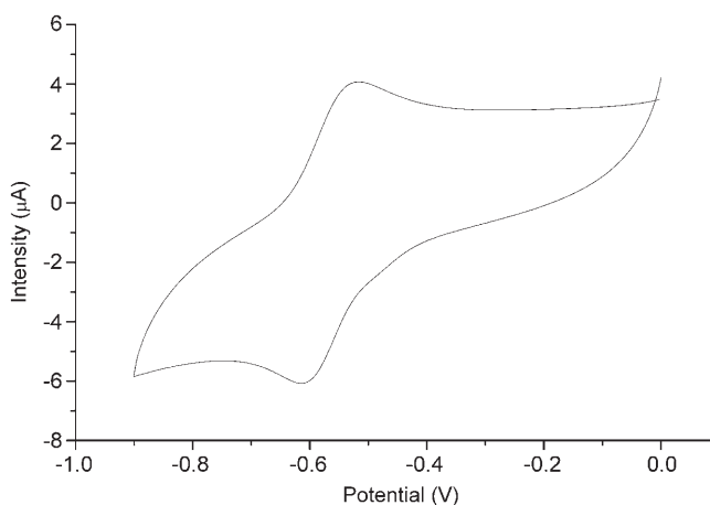
Figure 2. Cyclic voltammogram of \text{Fe}^{\text{III}} -EDDHA. Conditions: [\text{FeCl}_3 \cdot 6\text{H}_2\text{O}] 10^{-3}\text{ M} , [o,o\text{-EDDHA}] 10^{-2}\text{ M} , pH 7.4.
