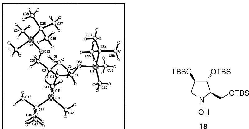
Figure 1. X-Ray structure of protected N -hydroxypyrrolidine 18
